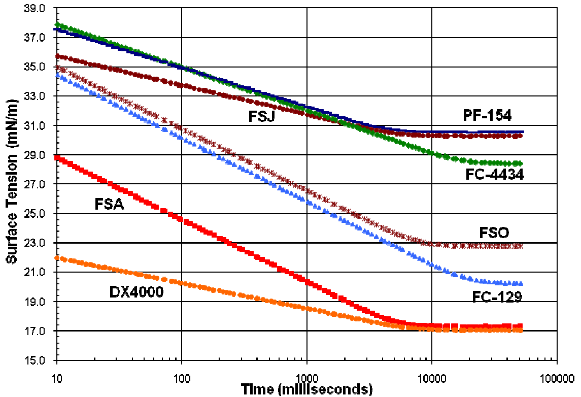
Fig. 2. Dynamic Surface Tensions of Competitive Fluorosurfactants at 0.01% Actives in Water
